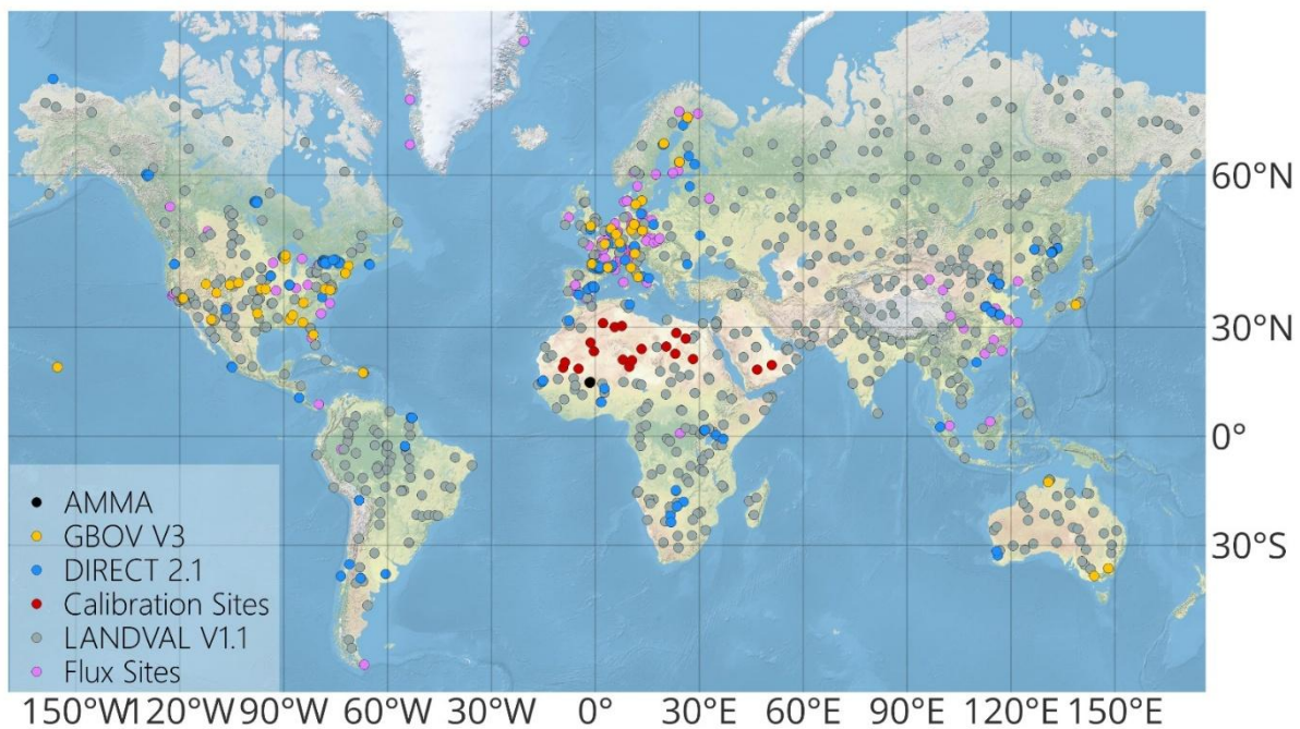
Figure 6: Selection of the sites for which 3x3 km LAI and fAPAR retrievals are available. The 1,122 sites correspond to a combination of Landval 1.1 (Fuster et al., 2020; Sánchez-Zapero et al., 2020), Calibration sites (Lacherade et al., 2013), GBOV (Brown et al., 2021), DIRECT 2.1 (Camacho et al., 2013), AMMA (Redelsperger et al., 2006) and Flux tower sites.
