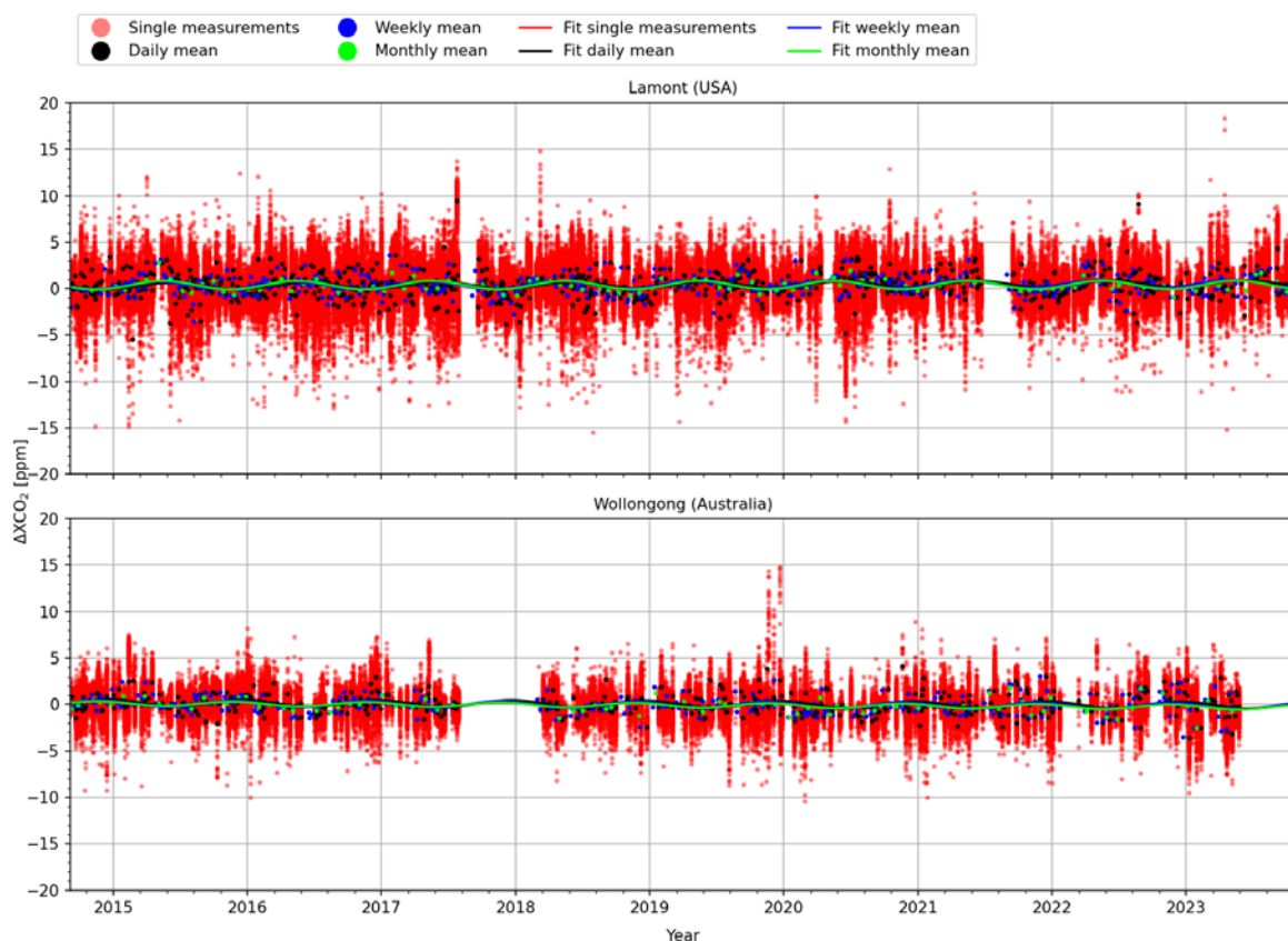
Figure 3.4: \Delta XCO_2 (FOCAL – TCCON) for the co-locations of the single measurements, daily, weekly, and monthly averages at the TCCON sites Lamont (top) and Wollongong (bottom). Additionally, the corresponding fits of the bias model (Eq. 3-1) are shown.
