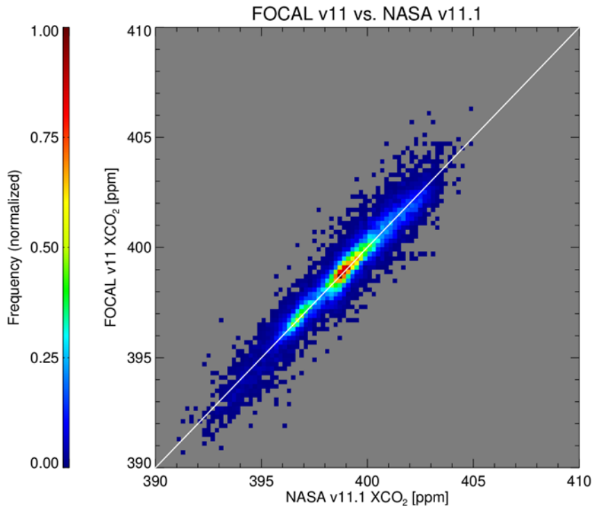
Figure 5.2: Heat map of FOCAL vs. NASA OCO-2 v11.1 XCO 2 data on the basis of monthly mean 5°x5° grid boxes including more than 100 data points.
