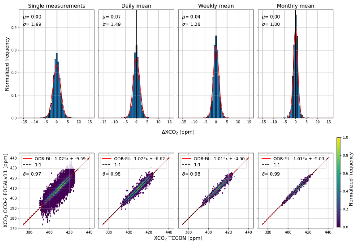
Figure 3.3: Overall overview on the agreement of the FOCAL data (and its averages) with TCCON data at all sites. Top: Normalized histograms of the difference FOCAL – TCCON. Bottom: Heat maps TCCON vs. FOCAL including one-to-one line, orthogonal distance regression (ODR), and Pearson correlation coefficient \delta .
