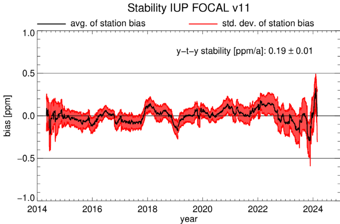
Figure 3.7: Stability analyses for FOCAL. The black curve shows the average station bias and the red curves its uncertainty represented by the station-to-station standard deviation
