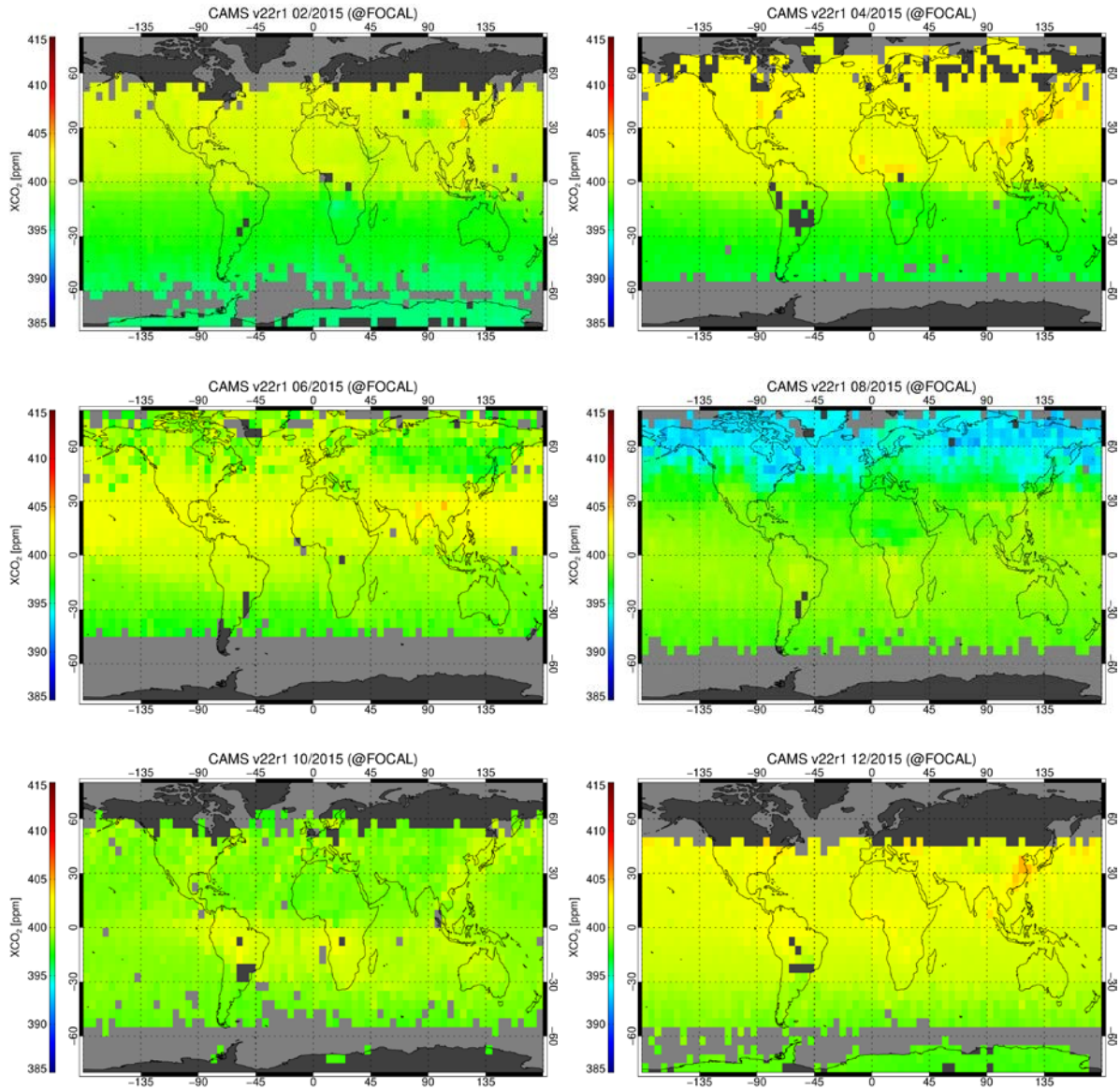
Figure 4.2: CAMS v22r1 monthly mean XCO 2 sampled as FOCAL and gridded to 5°x5°. From top/left to bottom/right: Feb., Apr., Jun., Aug., Oct., and Dec. 2015.
