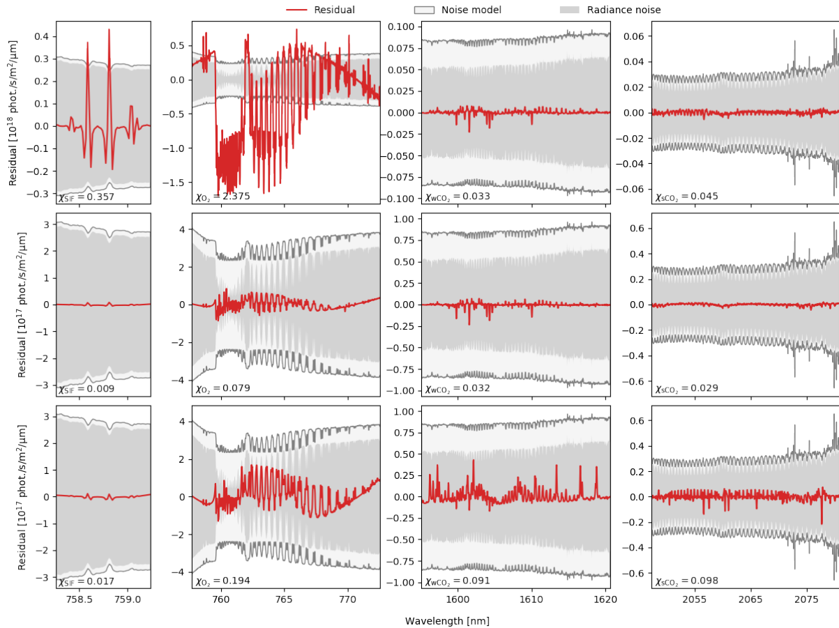
Figure 2.2: Residuals (fit minus measurement, red) and measurement noise (gray area = noise expected from the OCO-2 instrument, gray line = FOCAL's noise model used for the retrieval /ATBDv5, 2024/) of SCIATRAN simulated OCO-2 measurements fitted with FOCAL (solar zenith angle = 40°, parallel polarization). Top: Rayleigh scenario but with disabled fitting of scattering parameters. Middle: Rayleigh scenario. Bottom: Rayleigh+Aerosol BG+Water cloud scenario. See also /Reuter et al., 2017a/ for details on the geophysical scenarios and /ATBDv5, 2024/ for details on the retrieval setup.
