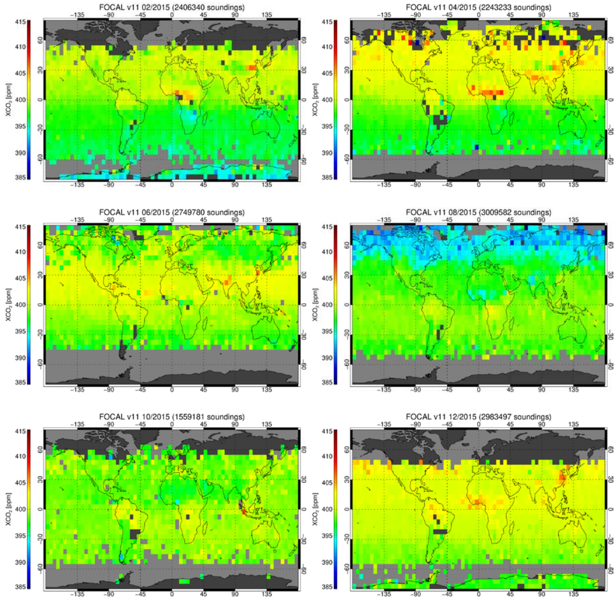
Figure 4.1: FOCAL v11 monthly mean XCO 2 gridded to 5°×5°. From top/left to bottom/right: Feb., Apr., Jun., Aug., Oct., and Dec. 2015.
