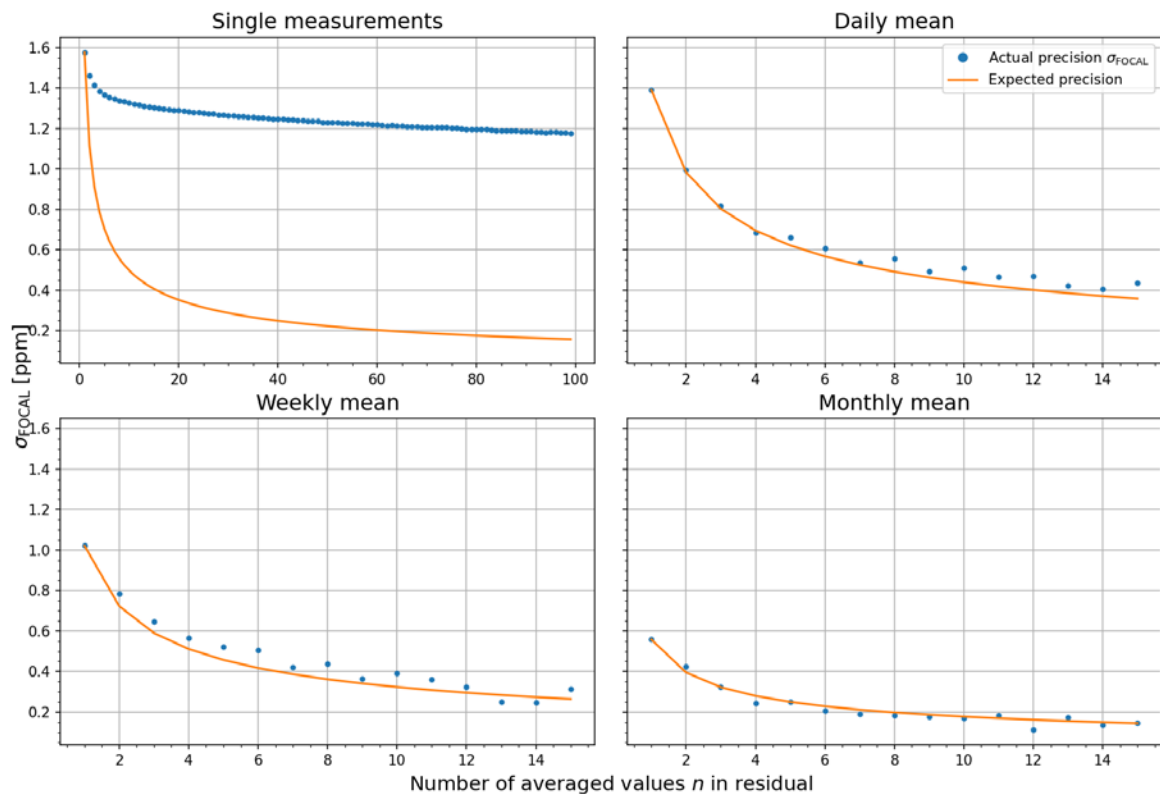
Figure 3.6: Actual and expected retrieval precision of FOCAL computed from residuals with increasing bin size for the TCCON site Lamont for single measurements (top/left), daily (top/right), weekly (bottom/left), and monthly averages (bottom/right).
