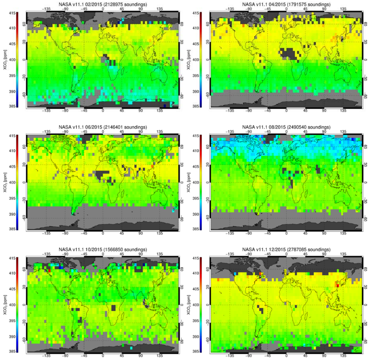
Figure 5.1: NASA's operational OCO-2 v11.1 XCO 2 L2 product gridded to 5°x5° monthly means. From top/left to bottom/right: Feb., Apr., Jun., Aug., Oct., and Dec. 2015.
