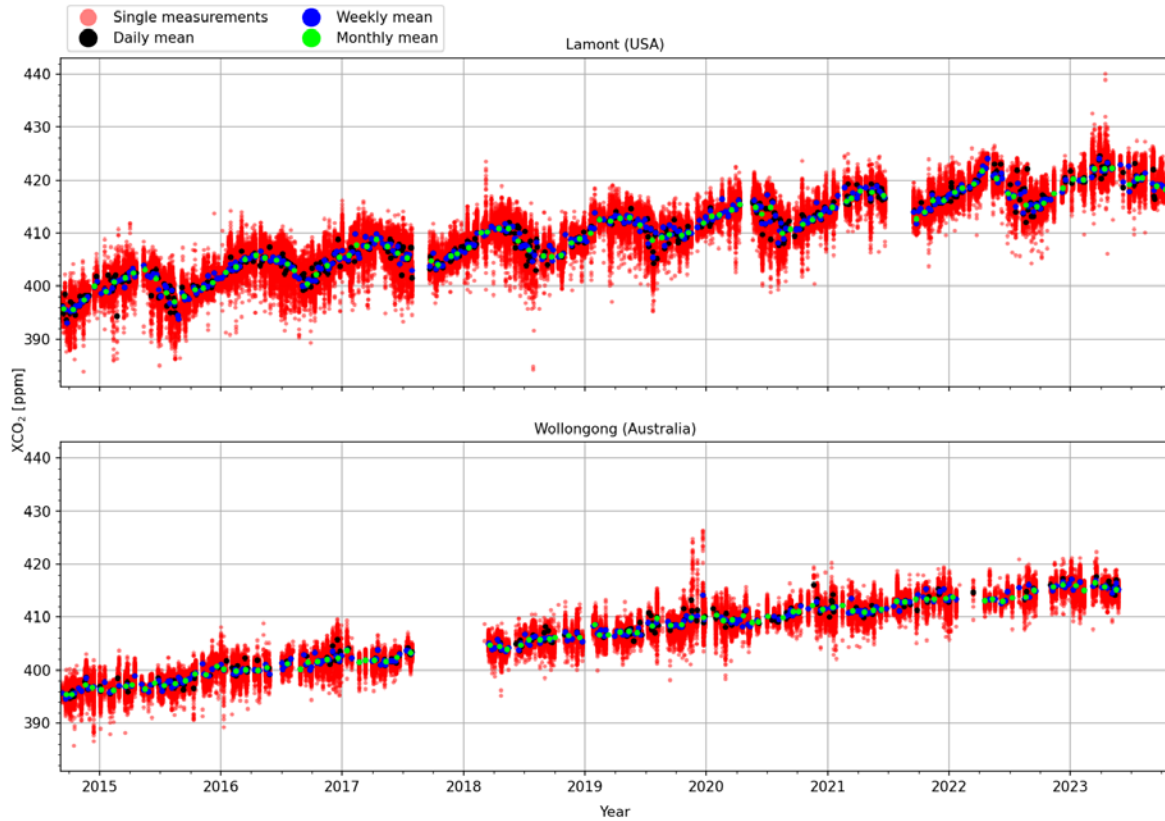
Figure 3.2: Co-located FOCAL XCO 2 retrieval results and their daily, weekly, and monthly averages at the TCCON sites Lamont (top) and Wollongong (bottom) used for the validation study.
